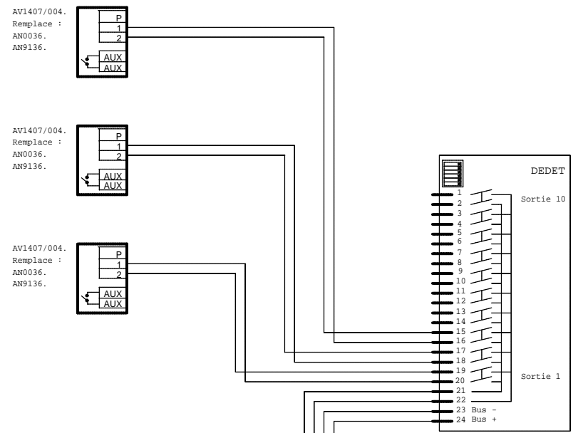
PLATINE A DEFILIEMENT UAV0153/112
