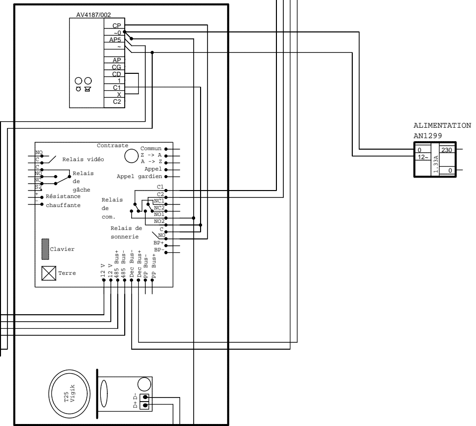
PLATINE A DEFILIEMENT UAV0153/112
